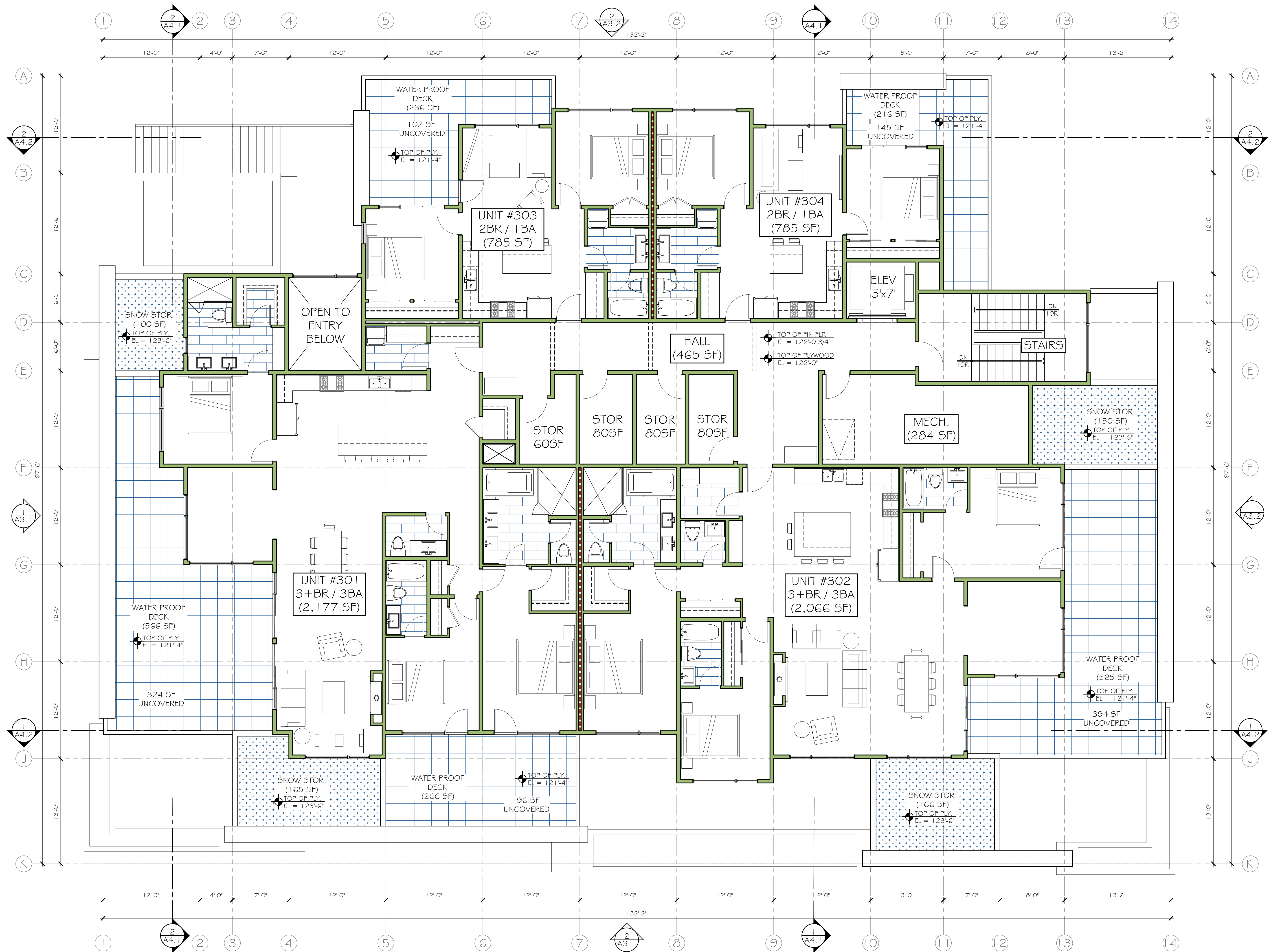
1 A2.3 THIRD LEVEL FLOOR PLAN SCALE: 3/16" = 1'-0"
