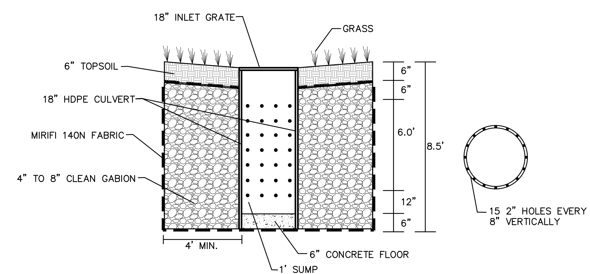
TYPICAL INFILTRATION AREA DETAIL
