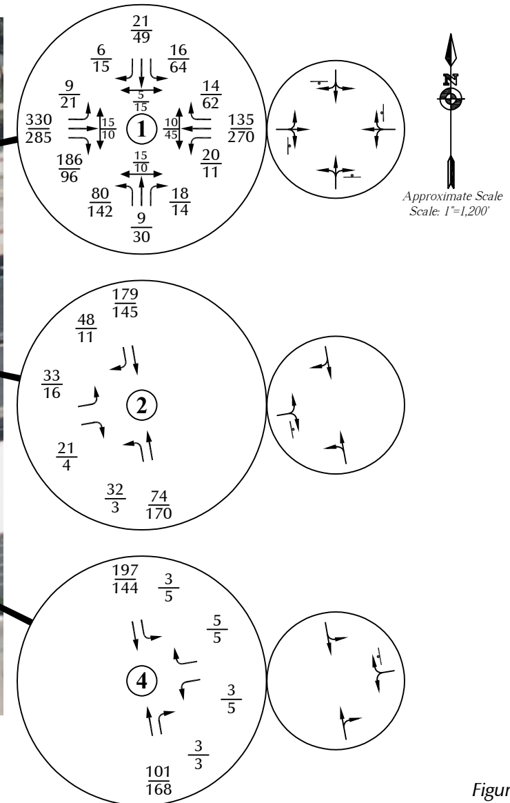
Year 2045 Background Traffic, Lane Geometry and Traffic Control
