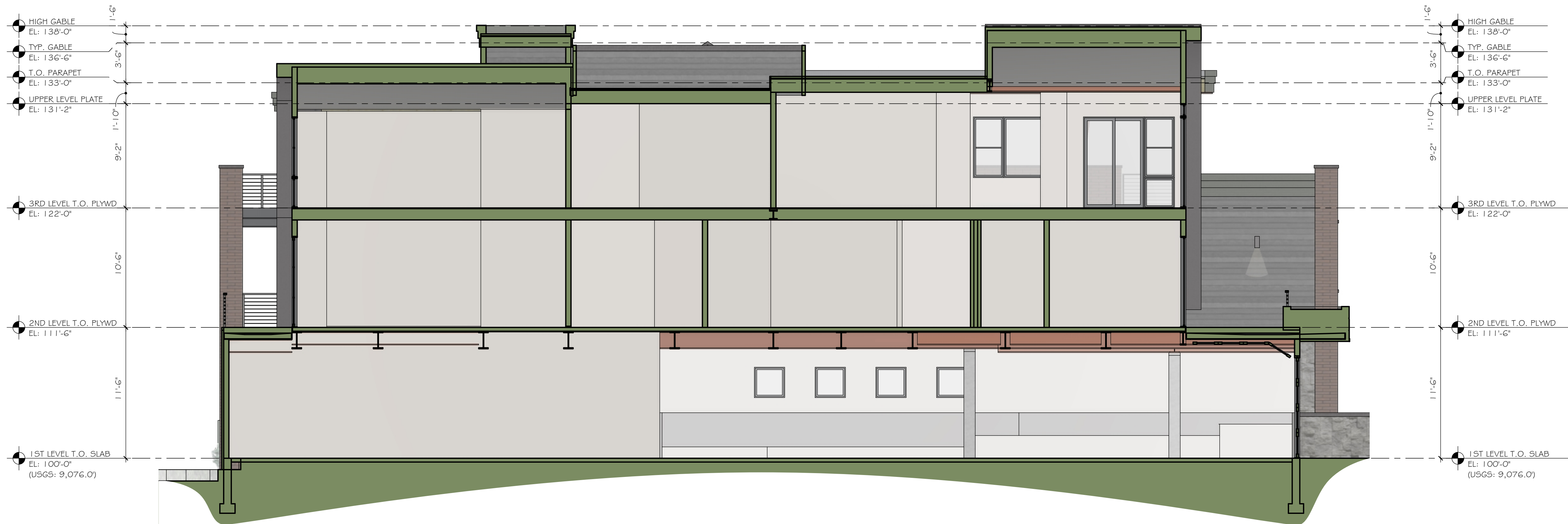
1 A4.1 BUILDING SECTION 3/16" = 1'-0"
